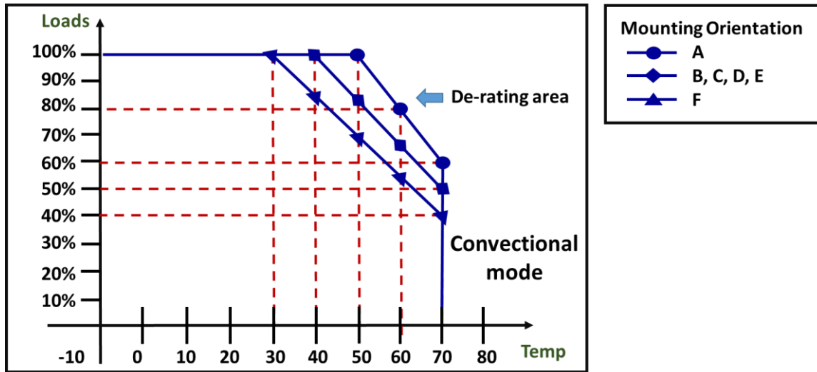
Note: De-rating Power Output with Temperature
